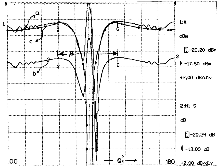
Fig. 1. The transmittance curves for window glass at 8 GHz. a —experimentally measured, b —the same curve a , but smoothed by 2%. c —theoretically calculated for comparison using (2).
