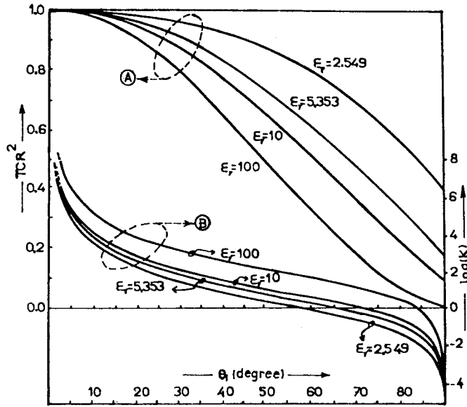
Fig. 2. Theoretical curves for different values of \epsilon_r . (A)— \text{TCR}^2 versus \theta_1 . (B)— \log(K) versus \theta_1 (intersection of the curves with the x -axis is the relative pseudo-Brewster's angle).
